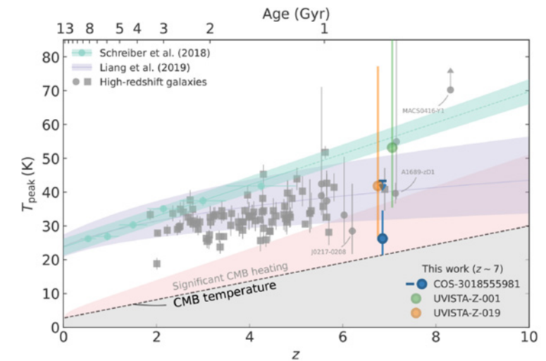
Fig. 2: Dust peak temperature, T_{\text{peak}} , as a function of cosmic time or redshift. Sources studied in this work are shown in colour, one of which has a notably low temperature. Figure from Witstok et al. (2022).
