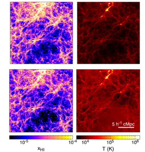
Fig. 2: Effects of homogeneous (top row) and inhomogeneous (bottom row) cosmic reionization on the neutral-hydrogen fraction (left) and gas temperature (right). The underdense regions become ionised later and exhibit higher temperatures in the model of inhomogeneous reionization. The neutral fractions of the gas are also lower in the filamentary structures of the cosmic web as the flux of ionising radiation is greater in higher-density regions hosting more sources of ionising radiation from the first galaxies and stars.
