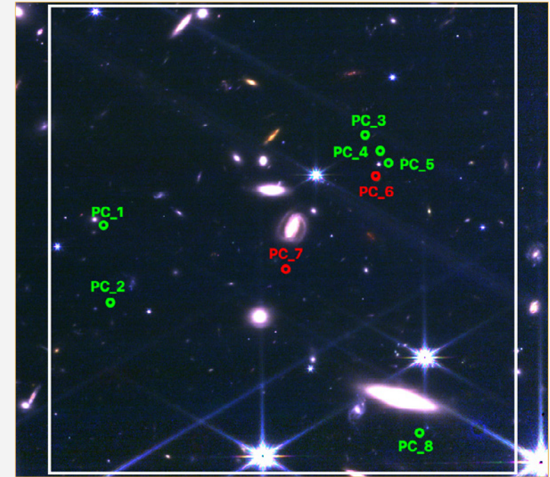
Fig. 1: Positions of all the protocluster’s members within a 40 arcsec by 40 arcsec region (white square). Green circles indicate the positions of galaxies with similar colours, while red circles show galaxies with measured redshifts of z = 7.66 .
