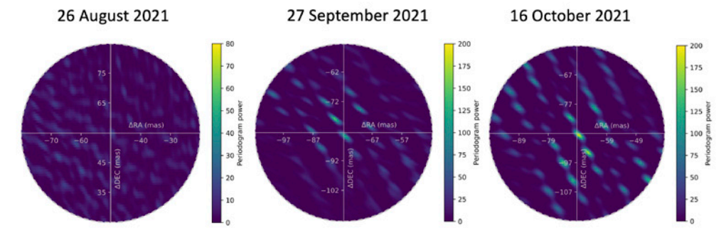
Fig. 1: Interferometric observations of HD 206893 c. Each plot represents the periodogram power in the limited field-of-view of GRAVITY. Nothing was detected in August, but a clear detection is visible in September and October.
